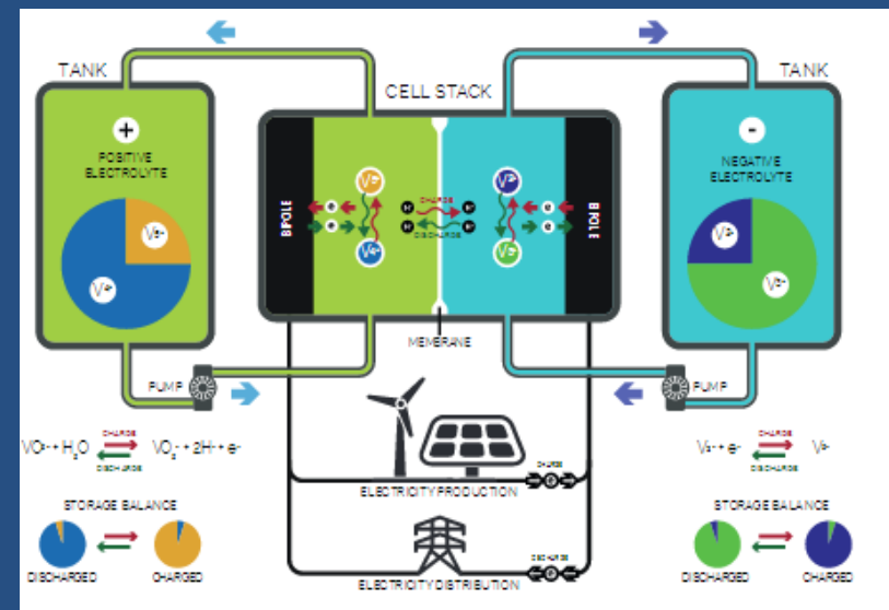
VRB BATTERY SCHEMATIC
